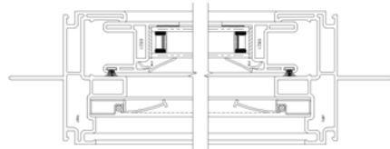
6 SASH JAMB SERIES 70 HUNG
