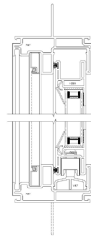
1 SASH HEAD SERIES 70 SLIDER
