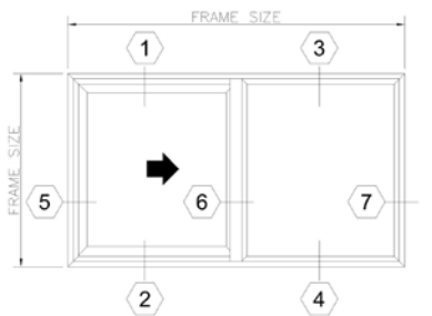
5 SASH JAMB SERIES 70 SLIDER 6 MTG RAIL SERIES 70 SLIDER 7 FIXED JAMB SERIES 70 SLIDER
