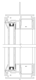
2 SILL SERIES 70 FIXED
